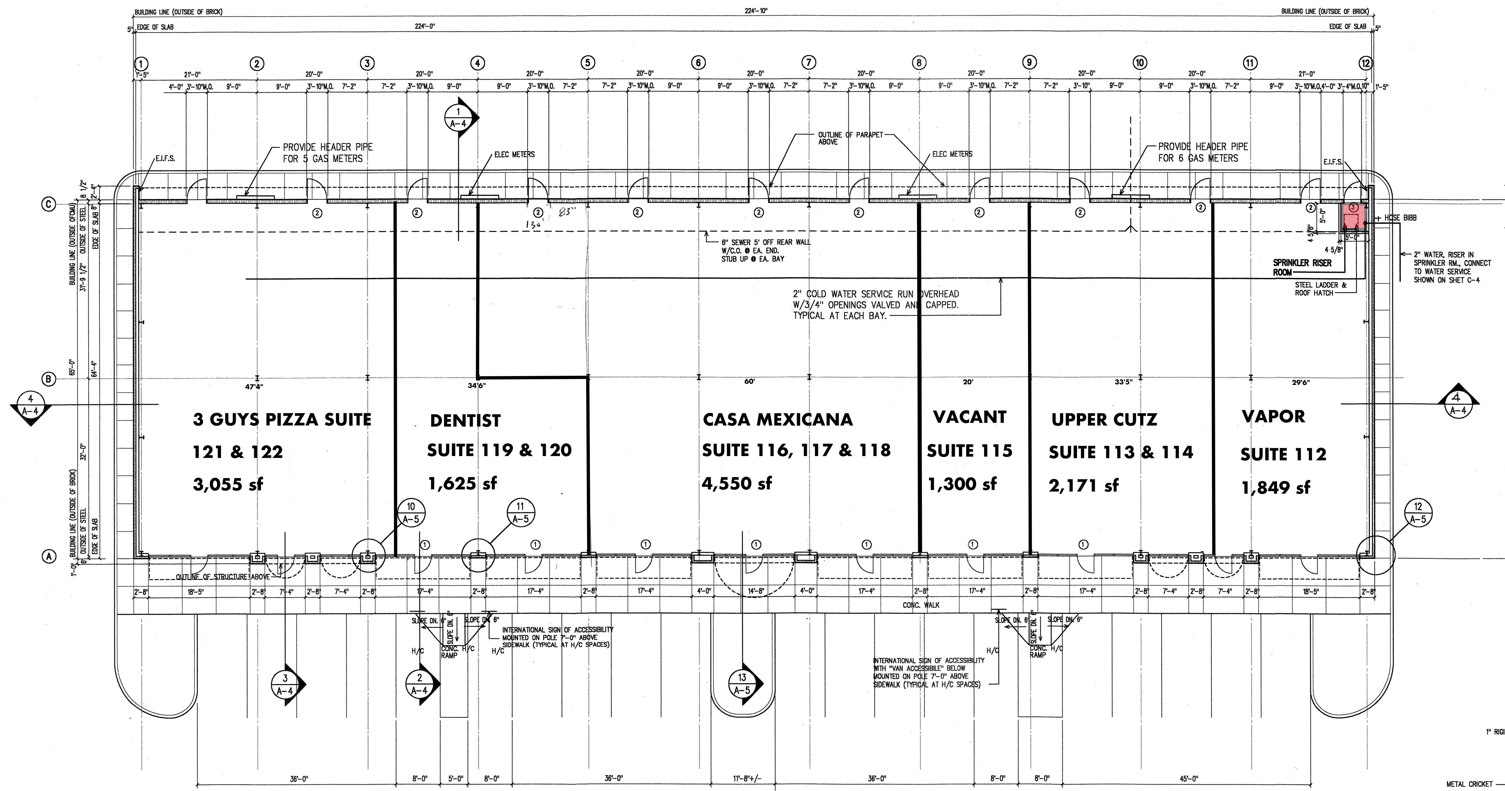
FLOOR PLAN 3/32" = 1'-0" N
